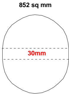
OVAL BORE VENTURI
